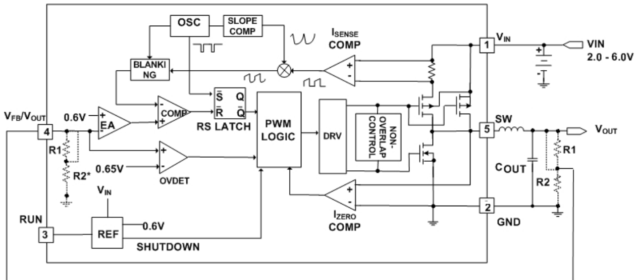
Figure 2. GX9216 Block Diagram
