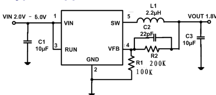
Figure 1. Basic Application Circuit with GX9216 adjustable version, V_{out} = 1.8V
