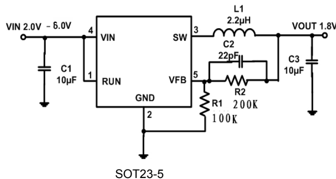
Figure 1. Basic Application Circuit with GX3410 adjustable version, V_{out} = 1.8V
