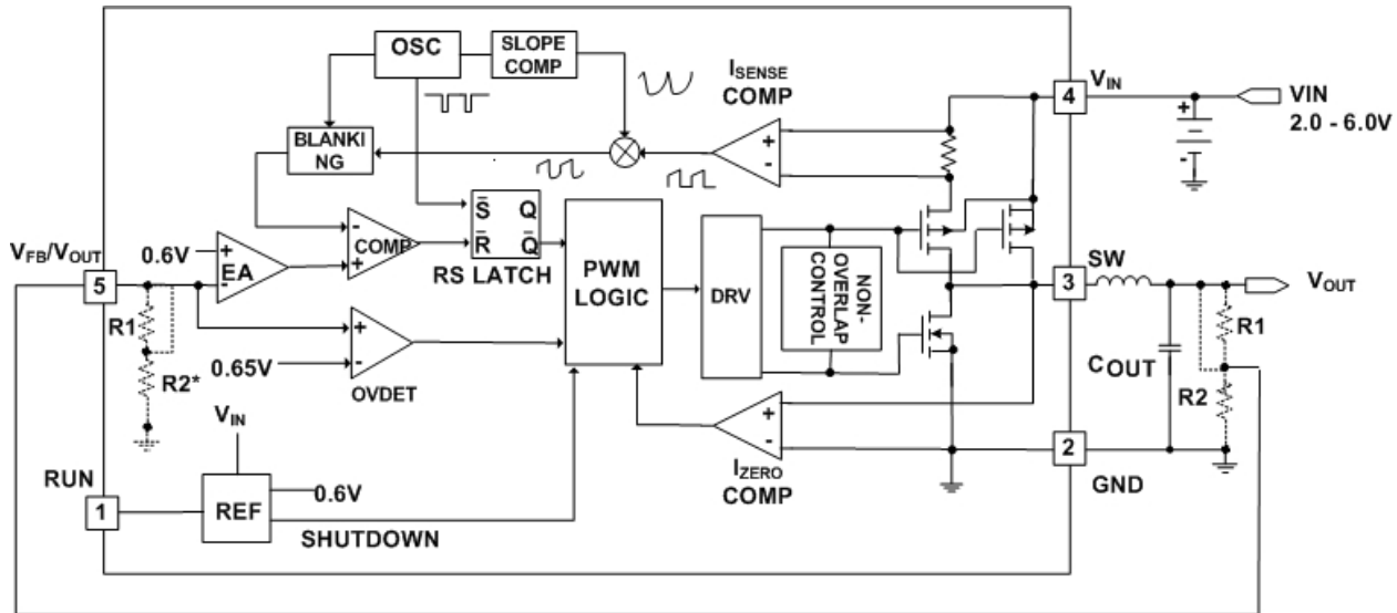
Figure 2. GX3410 Block Diagram
